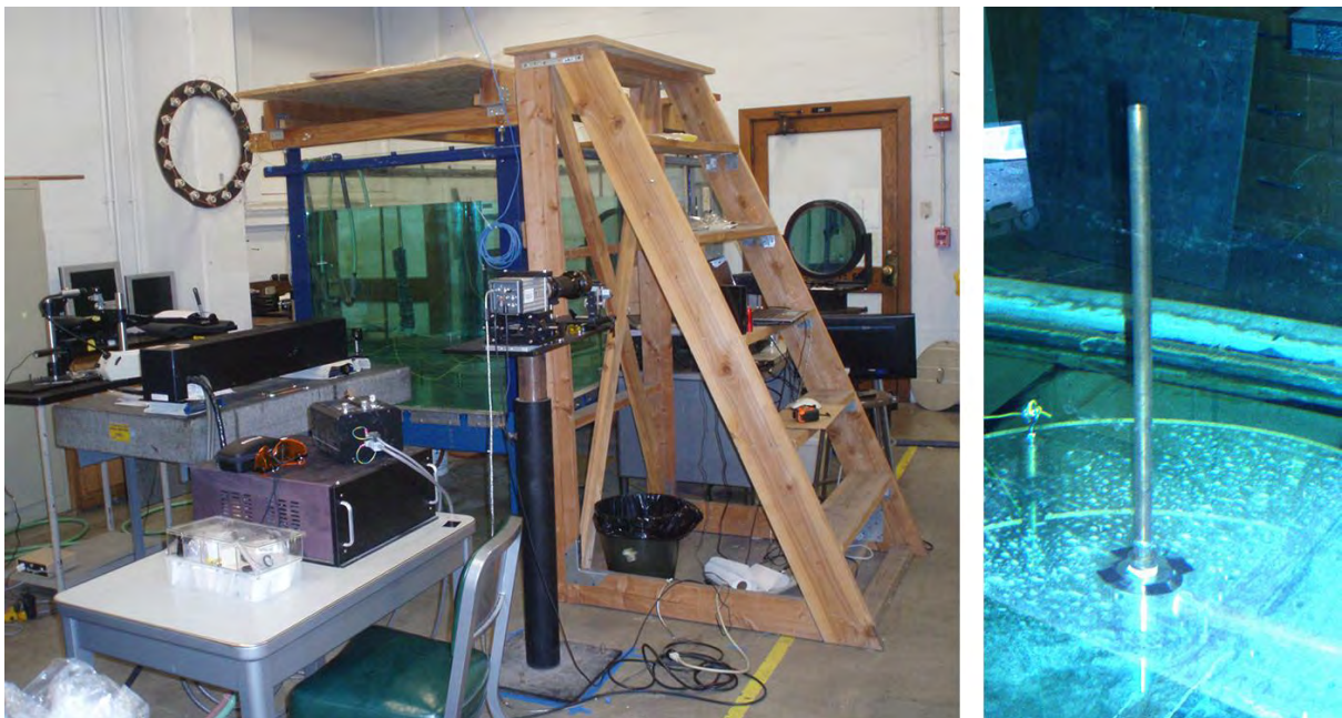
Figure 2. Overall view of the final setup (left) and the \frac{1}{2} inch diameter, 16 inches long discharge tube (right).
