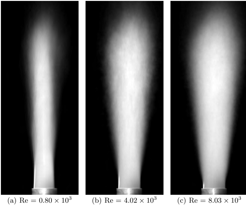
FIGURE 13. 5cs silicon oil jet experiments: intensity average 2048 images: Flows 24, 26 &amp; 29.
