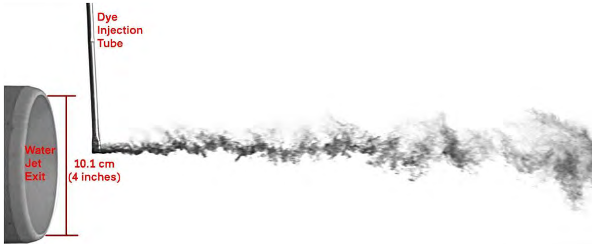
Figure 8. Flow visualization with dye point injection. Water flow rate was 41.7 liters/sec (11 gallons/sec) producing a Reynolds number of 500,000. The camera frame rate was 1500/second and the exposure time was 0.75 ms.
