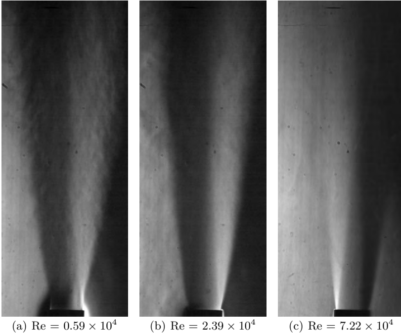
FIGURE 7. Schlieren of fluorescent water jet experiments: intensity average 2048 images: Flows 1, 3 & 6.
