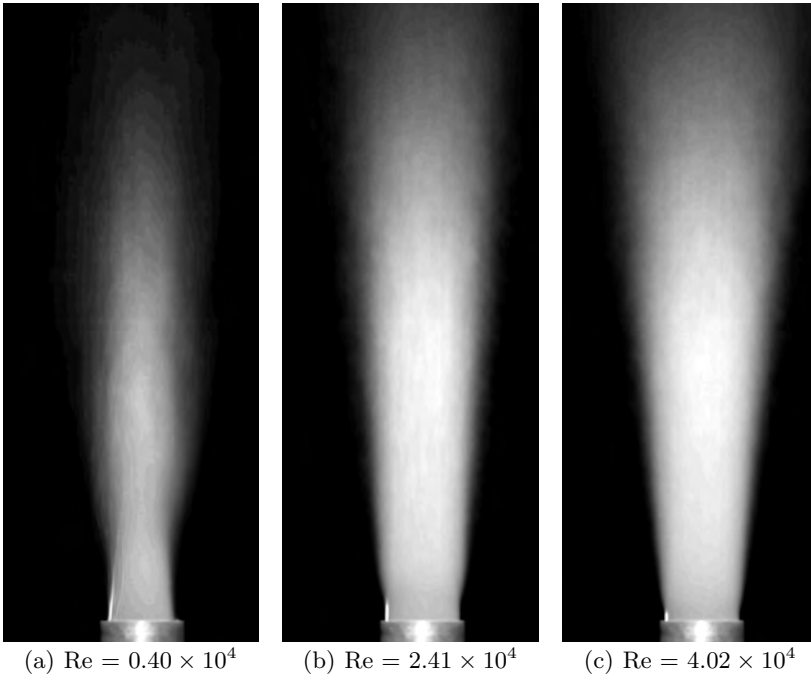
FIGURE 9. 1cs silicon oil jet experiments: intensity average 2048 images: Flows 19, 21 &amp; 23.
