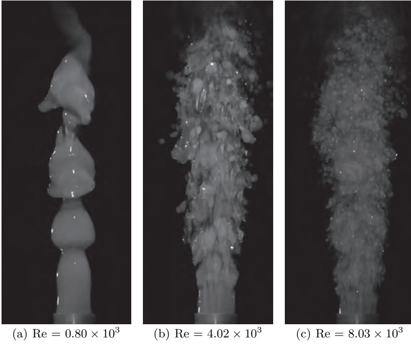
FIGURE 12. 5cs silicon oil jet experiments: Flows 24, 26 &amp; 29.
