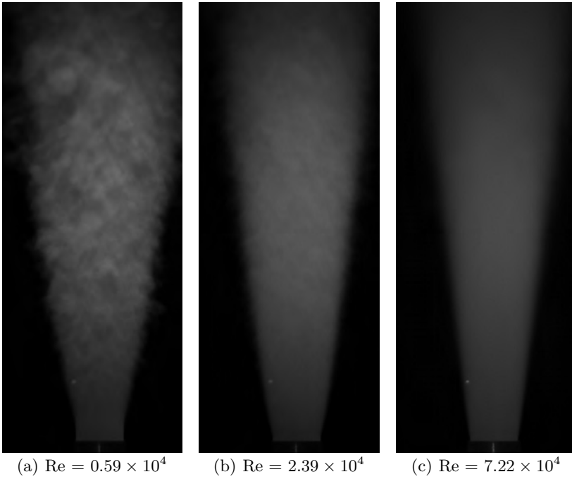
FIGURE 5. Fluorescent water jet experiments: intensity average 2048 images: Flows 1, 3 &amp; 6.
