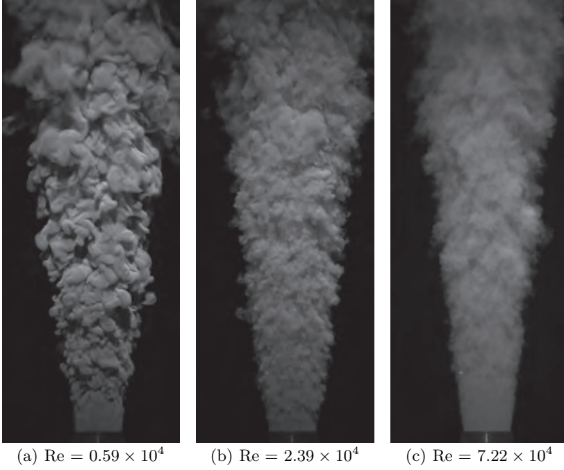
FIGURE 4. Fluorescent water jet experiments: Flows 1, 3 &amp; 6.
