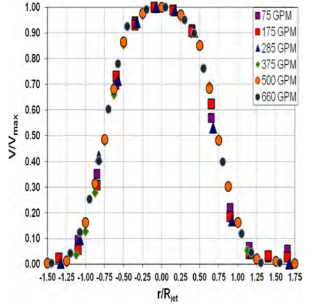
Fig. 10. Radial profiles of mean streamwise velocity measured with LDA for 10.1 cm diameter pipe jet at x=2.0D .
