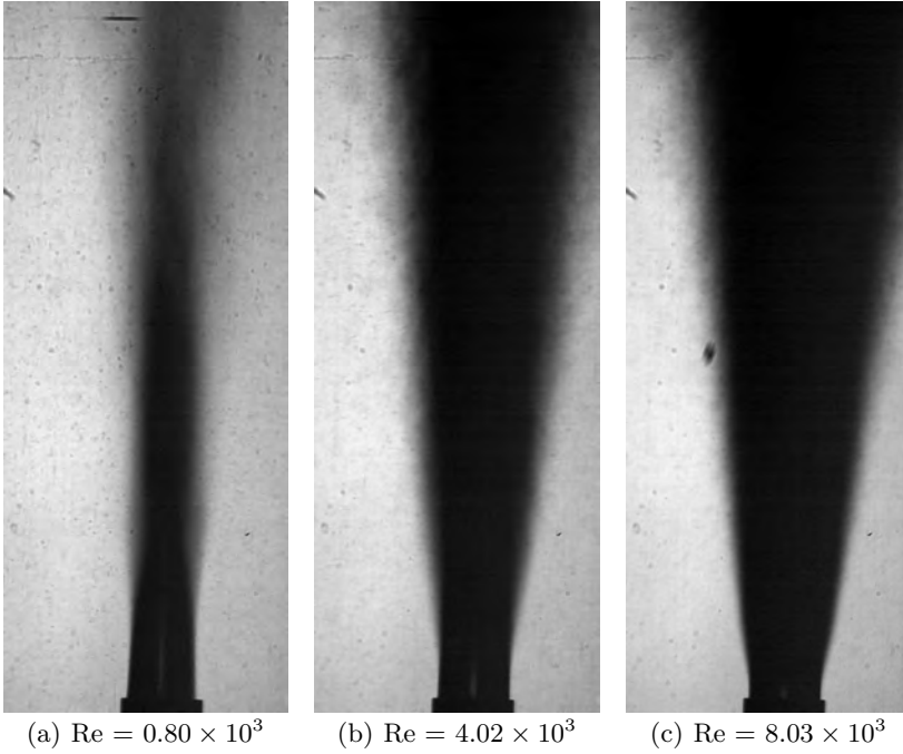
FIGURE 15. Shadowgraph of 5cs silicon oil jet experiments: intensity average 2048 images: Flows 24, 26 & 29.
