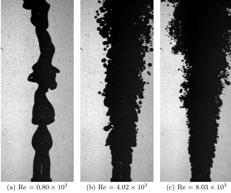
FIGURE 14. Shadowgraph of 5cs silicon oil jet experiments: Flows 24, 26 & 29.
