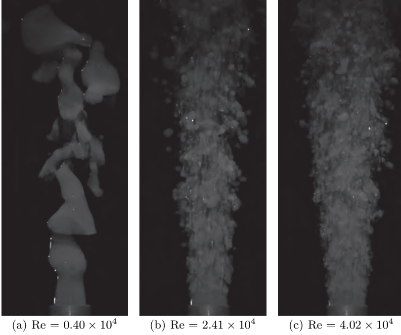
FIGURE 8. 1cs silicon oil jet experiments: Flows 19, 21 &amp; 23.
