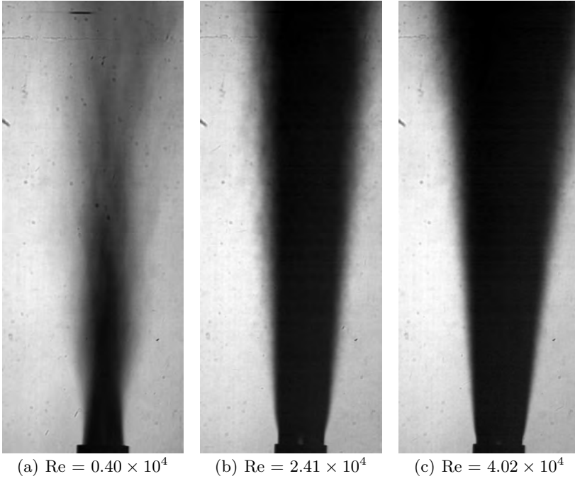
FIGURE 11. Shadowgraph of 1cs silicon oil jet experiments: intensity average 2048 images: Flows 19, 21 & 23.
