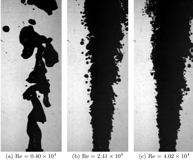
FIGURE 10. Shadowgraph of 1cs silicon oil jet experiments: Flows 19, 21 & 23.
